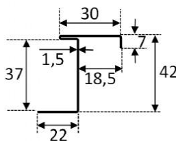
Panel Aluacero microperforado
